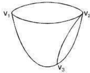
Un-Directed MultiGraph
