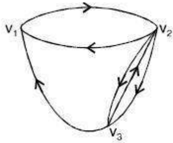
Directed MultiGraph
