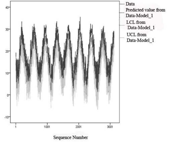
Fig. 8 Real and ARIMA system outputs related to temperature forecasting
