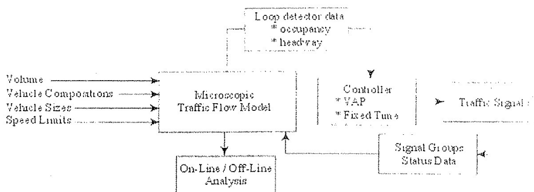
Figure 4- Flow chart about running a simulation process in VISSIM
