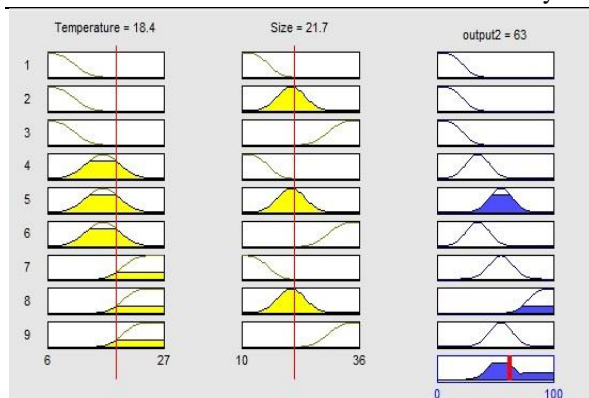
Figure 8. General rule viewer of proposed FLS.
